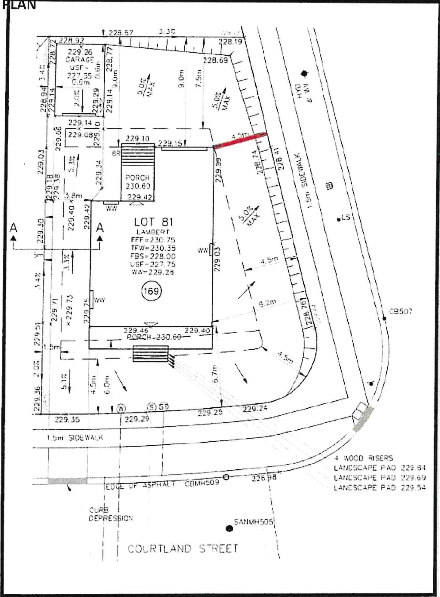
Excerpt of Lot 81 Plot Plan (Tatham Engineering)
