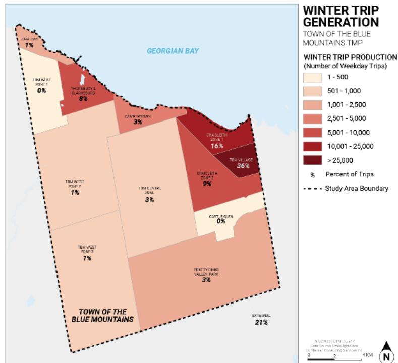
Figure 3-30 The Blue Mountains Internal Zones Trip Production in 2019 Winter Saturdays
