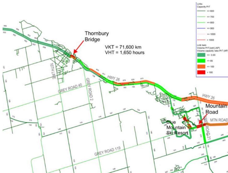
Figure 3-40: Winter Saturday Peak Hour Model Output (2019)
