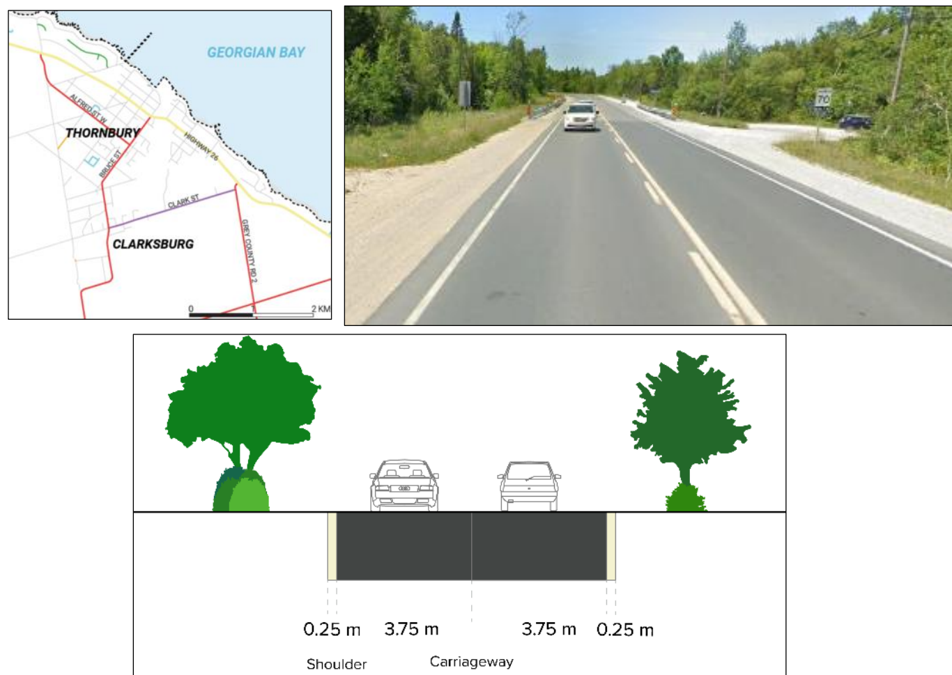
Figure 8-5: Existing Cross Section for Highway 26
