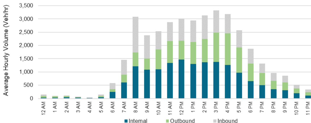
Figure 3-28: Average Hourly Trip Distribution (Fall Weekday, 2019)
