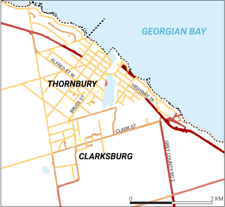
Figure 3-8: Existing Right-of-Way Widths in TBM
