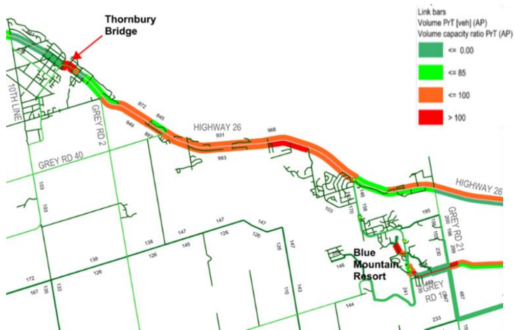
Figure 3-39: Summer Saturday Peak Hour Model Output (2019)
