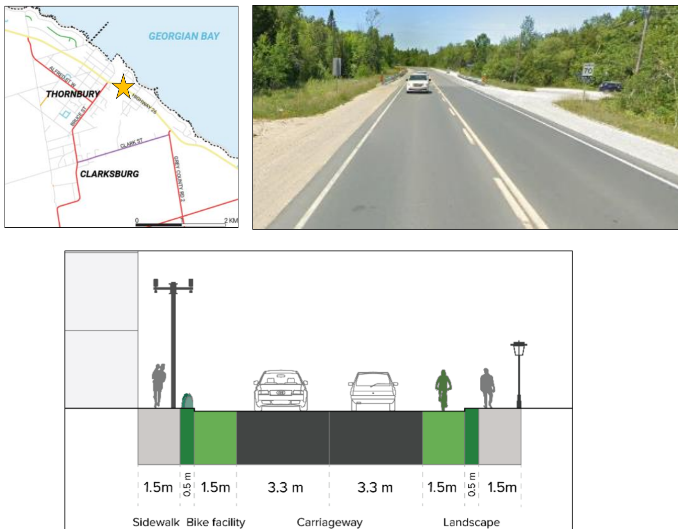
Figure 8-6: Potential Cross-Section Treatment for King Street
