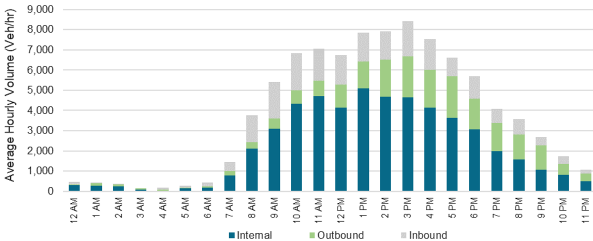
Figure 3-26: Average Hourly Trip Distribution (Winter Saturday, 2019)
