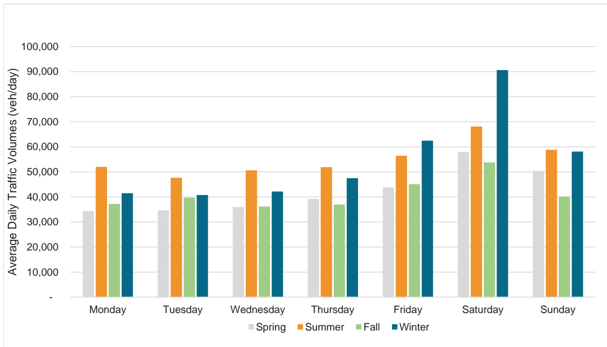
Figure 3-25: Seasonal Trip Frequency by Day of the Week (2019)
