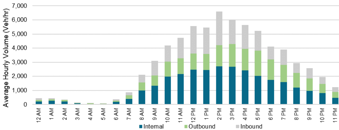
Figure 3-27: Average Hourly Trip Distribution (Summer Saturday, 2019)
