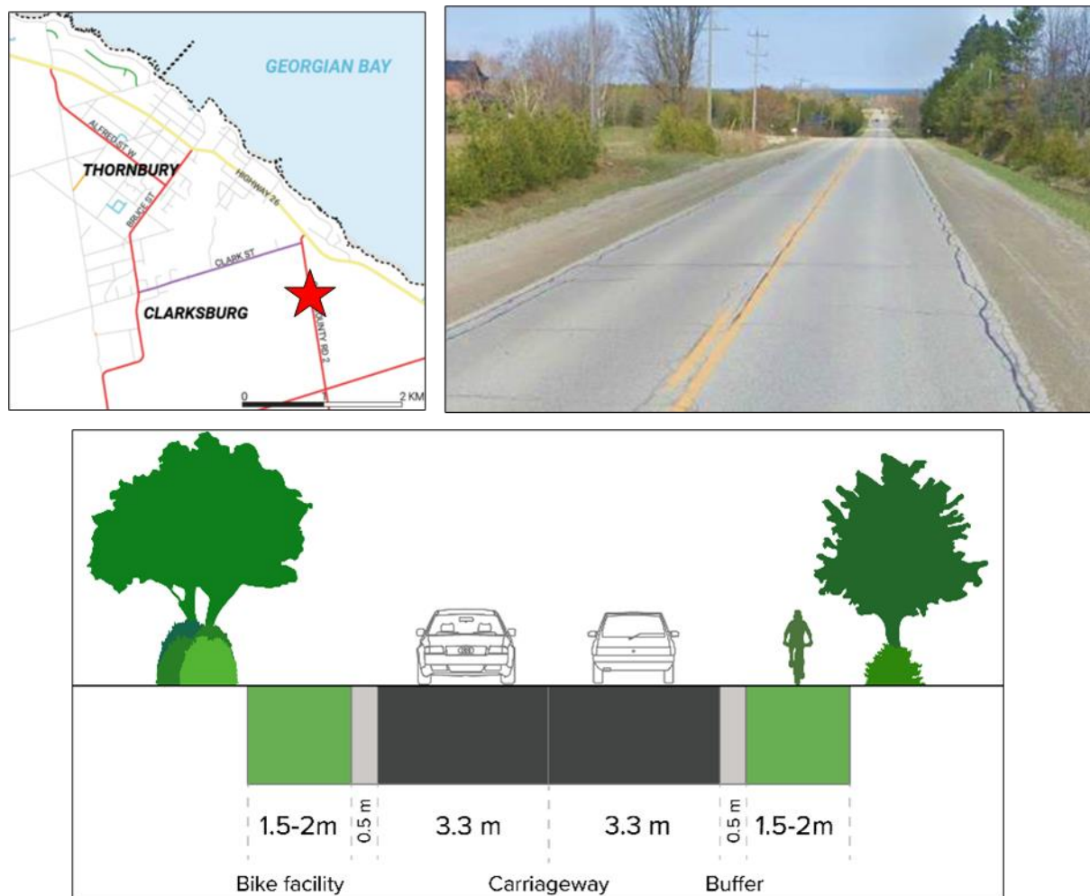
Figure 8-7: Potential Cross-Section Treatment for County Rd 2
