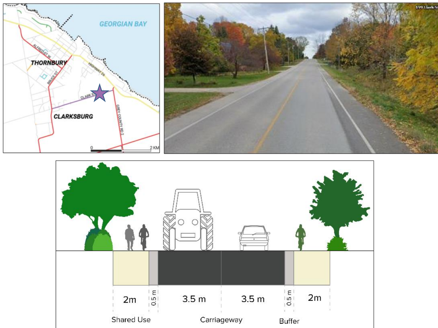
Figure 8-9: Potential Cross-Section Treatment for Clark Street
